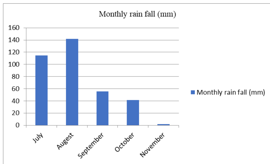
Supplementary Figure 2. Monthly rainfall amount at Miesso (2018).
