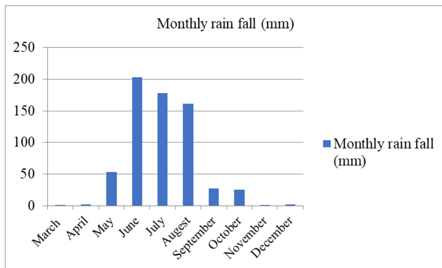
Supplementary Figure S1. Monthly rainfall amount at Sheraro (2018).
